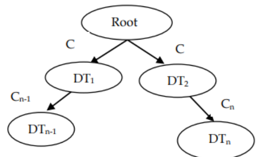
Fig. 4. Decision Tree
